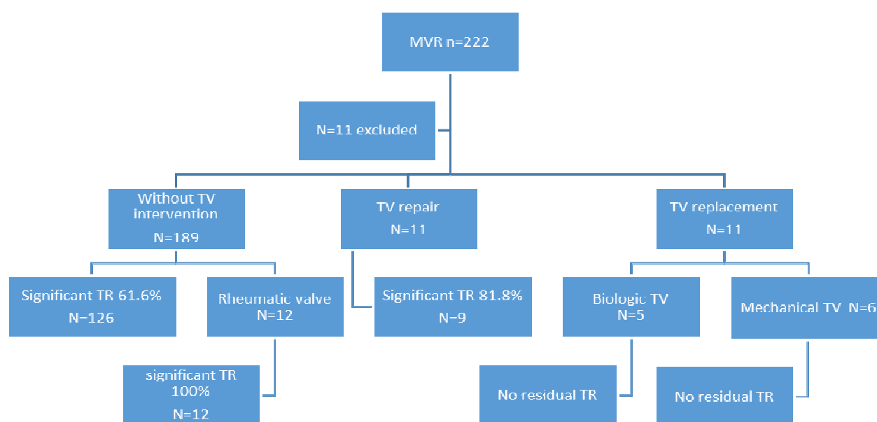
Figure 1. Study algorithm.
